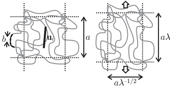
Fig. 1. Coarse-grained LCE model: undeformed ( left ) and stretched ( right ) unit cell (2D projection).
