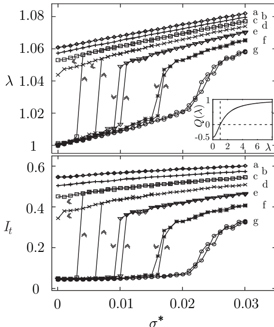
Fig. 2. Regular sample stretched: stress-strain isotherms ( top ) and light transmittance ( bottom ). Curves a-g correspond to T^* = 1.135 - 1.15 , with a step size of 0.0025. Arrows denote the scan direction; note the hysteresis. Inset: Q(\lambda) dependence.
