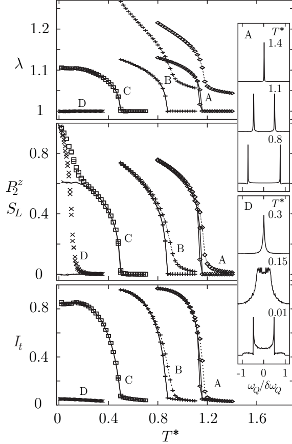
Fig. 3. Samples A-D: temperature scans. Sample length \lambda ( top ), P_2^z (lines) and S_L (symbols) order parameters ( center ), and transmittance I_t ( bottom ). No stress and \sigma^* = 0.1 (solid and dotted lines, respectively). Insets: ^2\text{H} NMR spectra for \sigma^* = 0 ; top : sample A, bottom : sample D.
